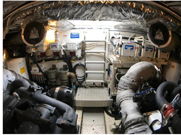
Engine Room Facing Aft
